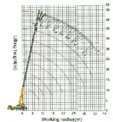
▲ Lifting height curves
